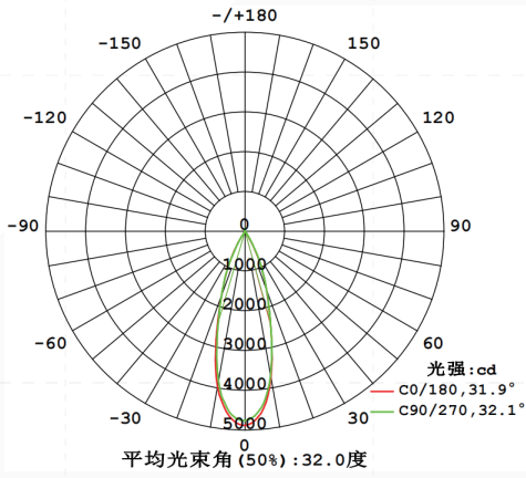
圆形格栅 30°
